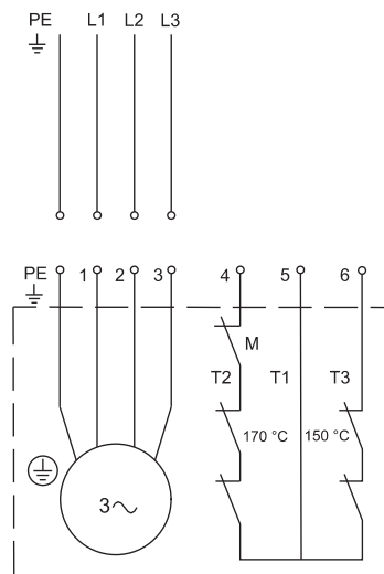
Wiring diagram for three-phase SEG pumps
