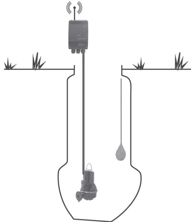
Pump(s) with CIU and level switch - Case 2
