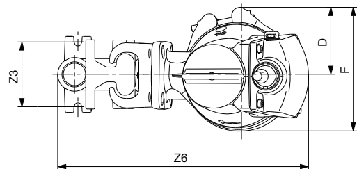
Installation on auto coupling
