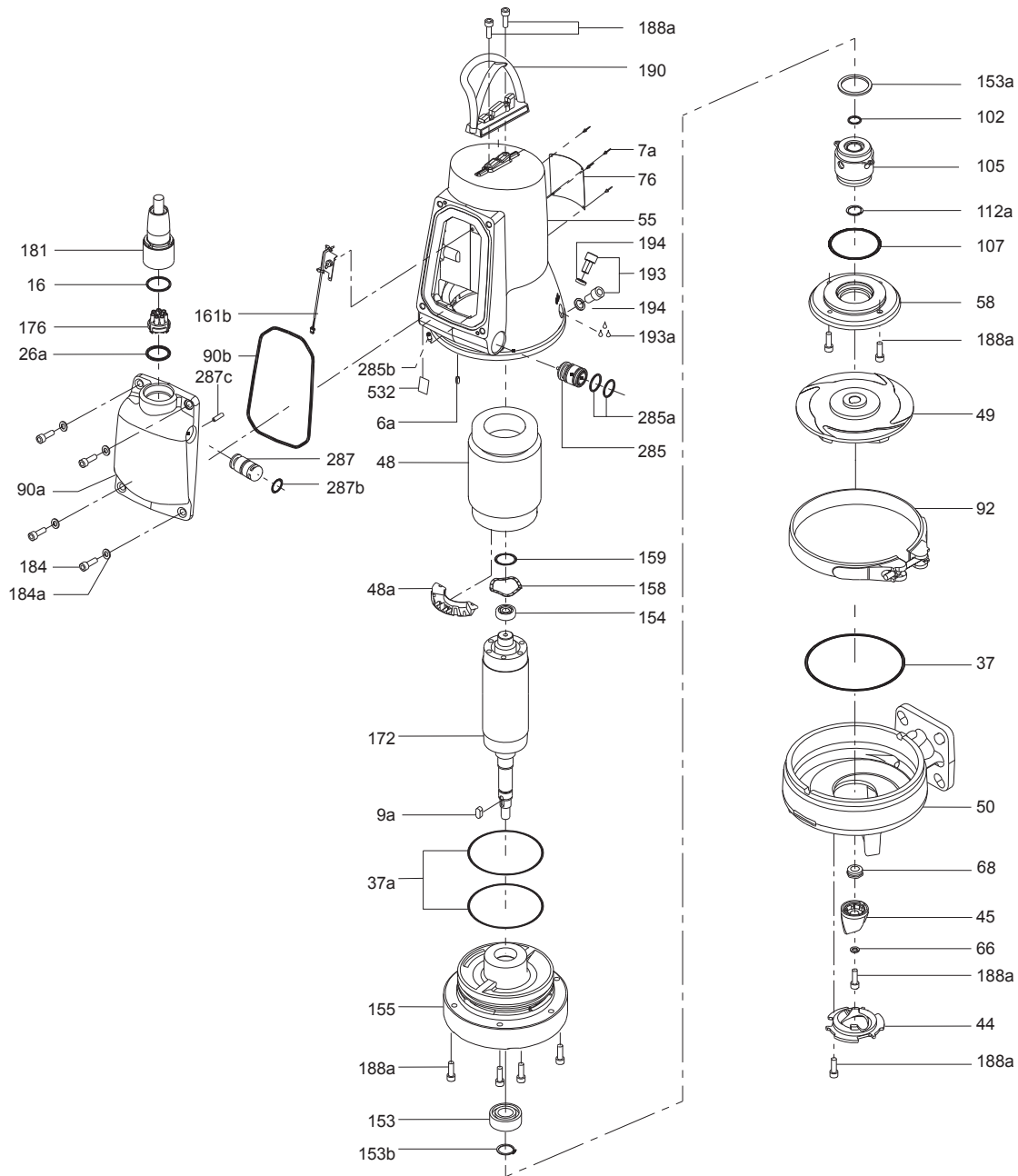
Exploded view of SEG AUTO ADAPT pumps, 2.6, 3.1 and 4.0 kW
