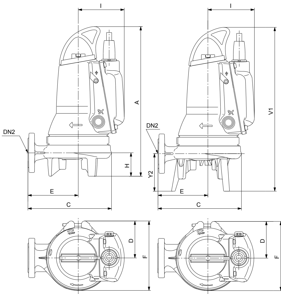
Free-standing installation with or without foot extensions
