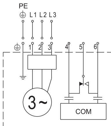
Wiring diagram for three-phase SEG AUTOADAPT pumps
