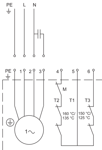
Wiring diagram for single-phase SEG pumps. See table below.
