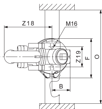
Installation on hookup auto coupling
