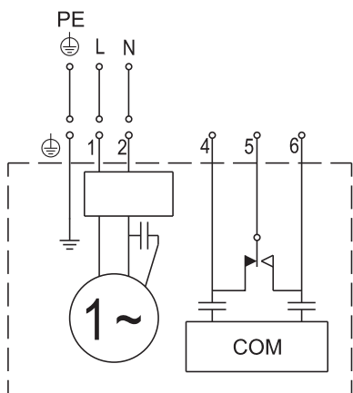
Wiring diagram for single-phase SEG AUTOADAPT pumps
