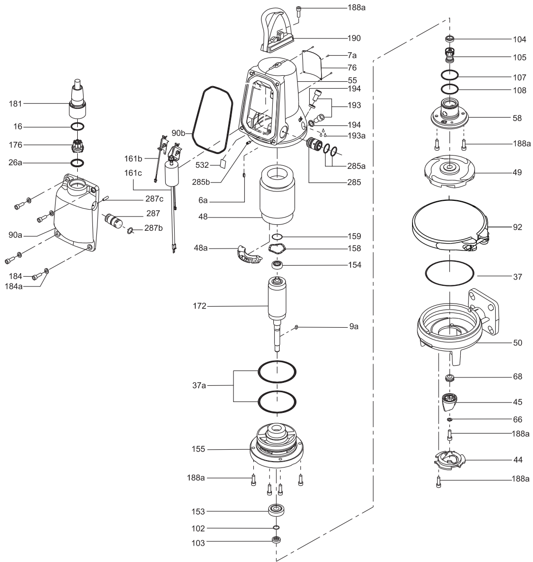
Exploded view of SEG AUTO ADAPT pumps, 0.9, 1.2 and 1.5 kW
